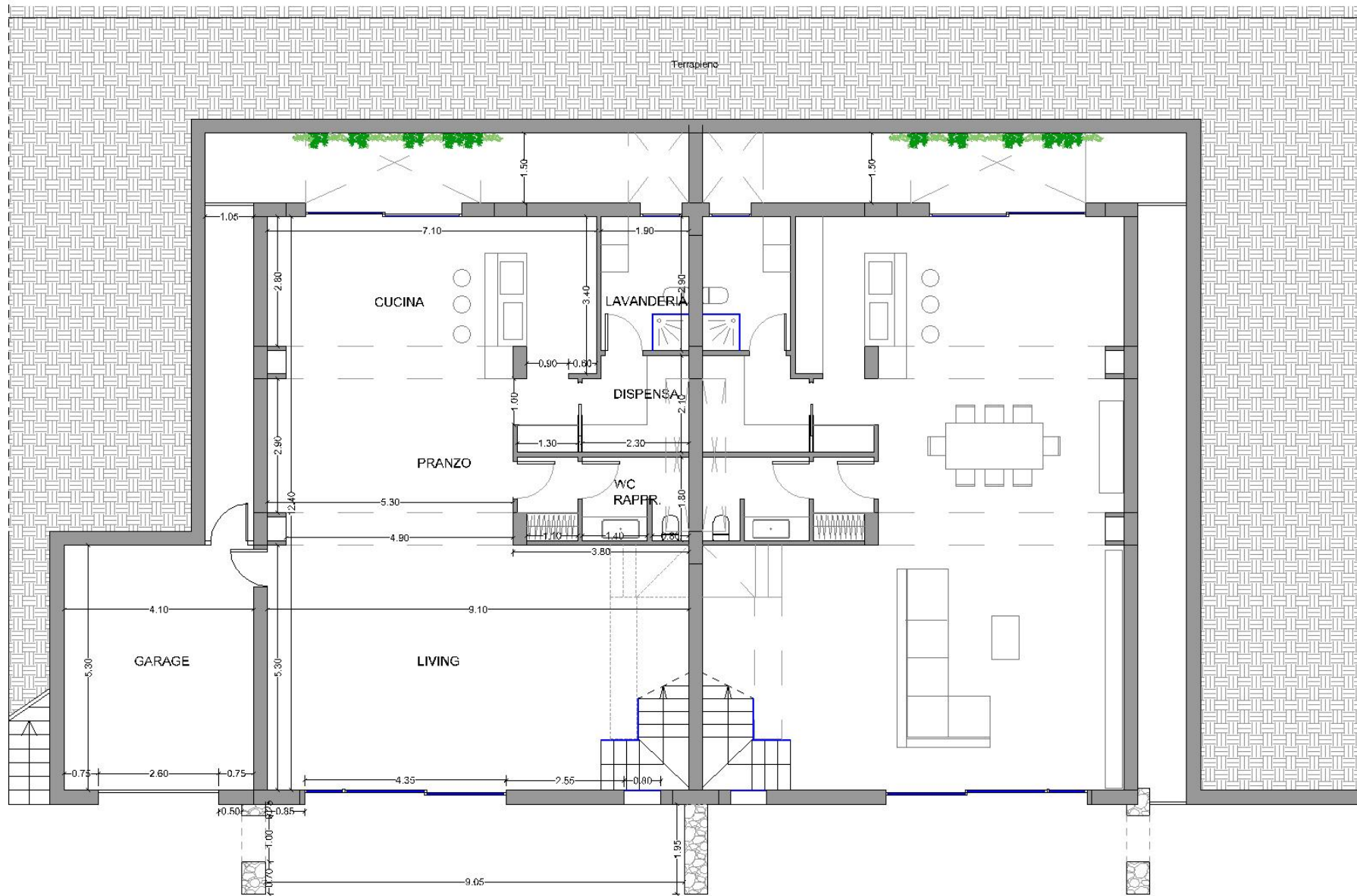
PIANTA PIANO -1
